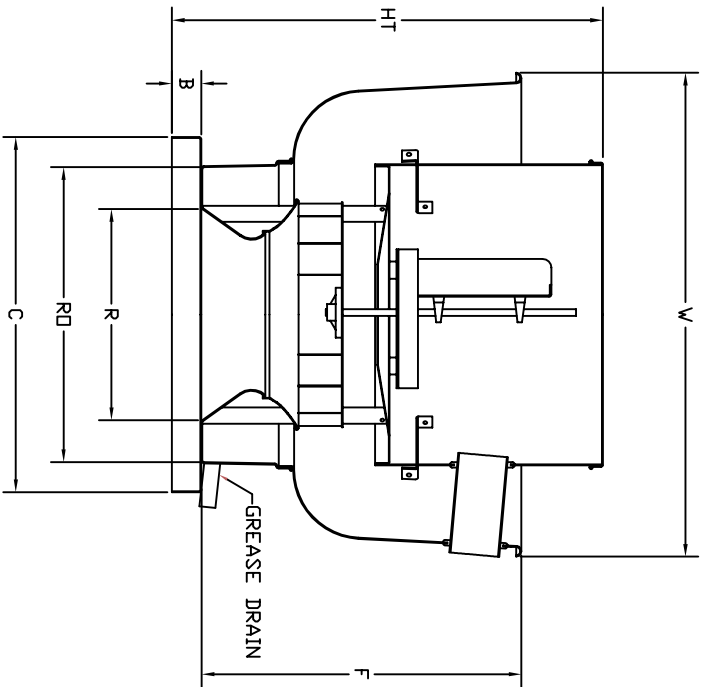
BDUHP BELT DRIVE CENTRIFUGAL UP-BLAST EXHAUST FANS DIMENSIONAL DATA
